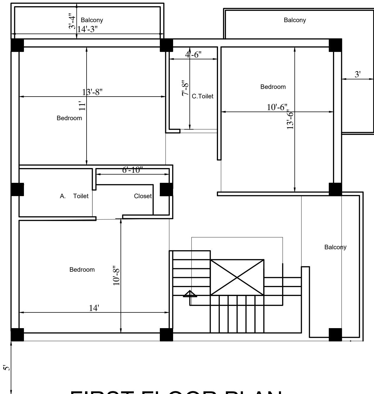
FIRST FLOOR PLAN AREA: 868.70 SQ. FT
